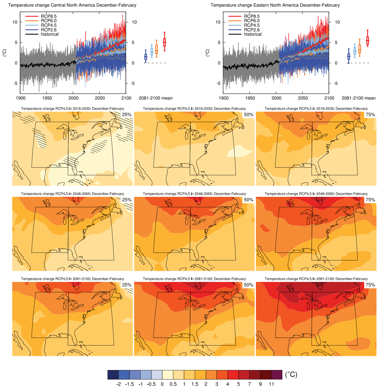
Figure AI.20 | (Top left) Time series of temperature change relative to 1986–2005 averaged over land grid points in Central North America (28.6°N to 50°N, 105°W to 85°W) in December to February. (Top right) Same for land grid points in Eastern North America (25°N to 50°N, 85°W to 60°W). Thin lines denote one ensemble member per model, thick lines the CMIP5 multi-model mean. On the right-hand side the 5th, 25th, 50th (median), 75th and 95th percentiles of the distribution of 20-year mean changes are given for 2081–2100 in the four RCP scenarios.
