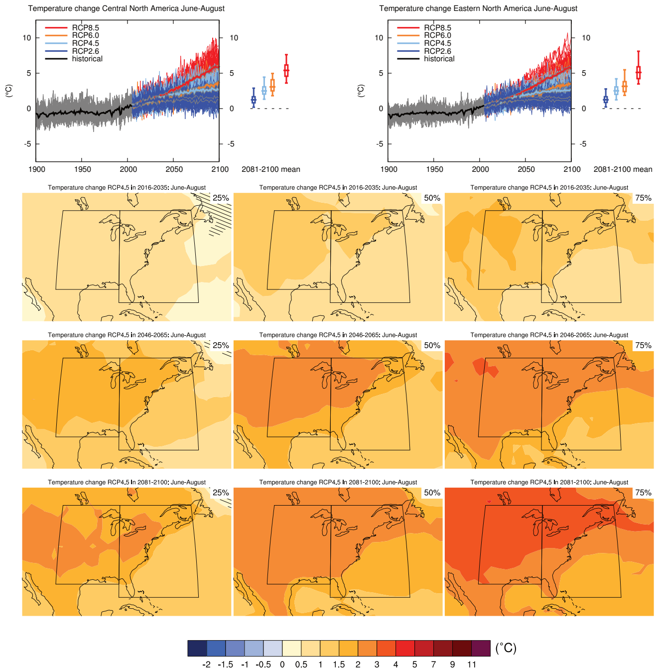
Figure AI.21 | (Top left) Time series of temperature change relative to 1986–2005 averaged over land grid points in Central North America (28.6°N to 50°N, 105°W to 85°W) in June to August. (Top right) Same for land grid points in Eastern North America (25°N to 50°N, 85°W to 60°W). Thin lines denote one ensemble member per model, thick lines the CMIP5 multi-model mean. On the right-hand side the 5th, 25th, 50th (median), 75th and 95th percentiles of the distribution of 20-year mean changes are given for 2081–2100 in the four RCP scenarios.
