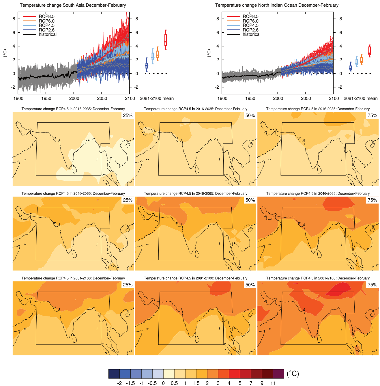
Figure AI.60 | (Top left) Time series of temperature change relative to 1986–2005 averaged over land grid points in South Asia (60°E, 5°N; 60°E, 30°N; 100°E, 20°E; 95°E, 20°N; 95°E, 5°N) in December to February. (Top right) Same for sea grid points in the North Indian Ocean (5°N to 30°N, 60°E to 95°E). Thin lines denote one ensemble member per model, thick lines the CMIP5 multi-model mean. On the right-hand side the 5th, 25th, 50th (median), 75th and 95th percentiles of the distribution of 20-year mean changes are given for 2081–2100 in the four RCP scenarios.
