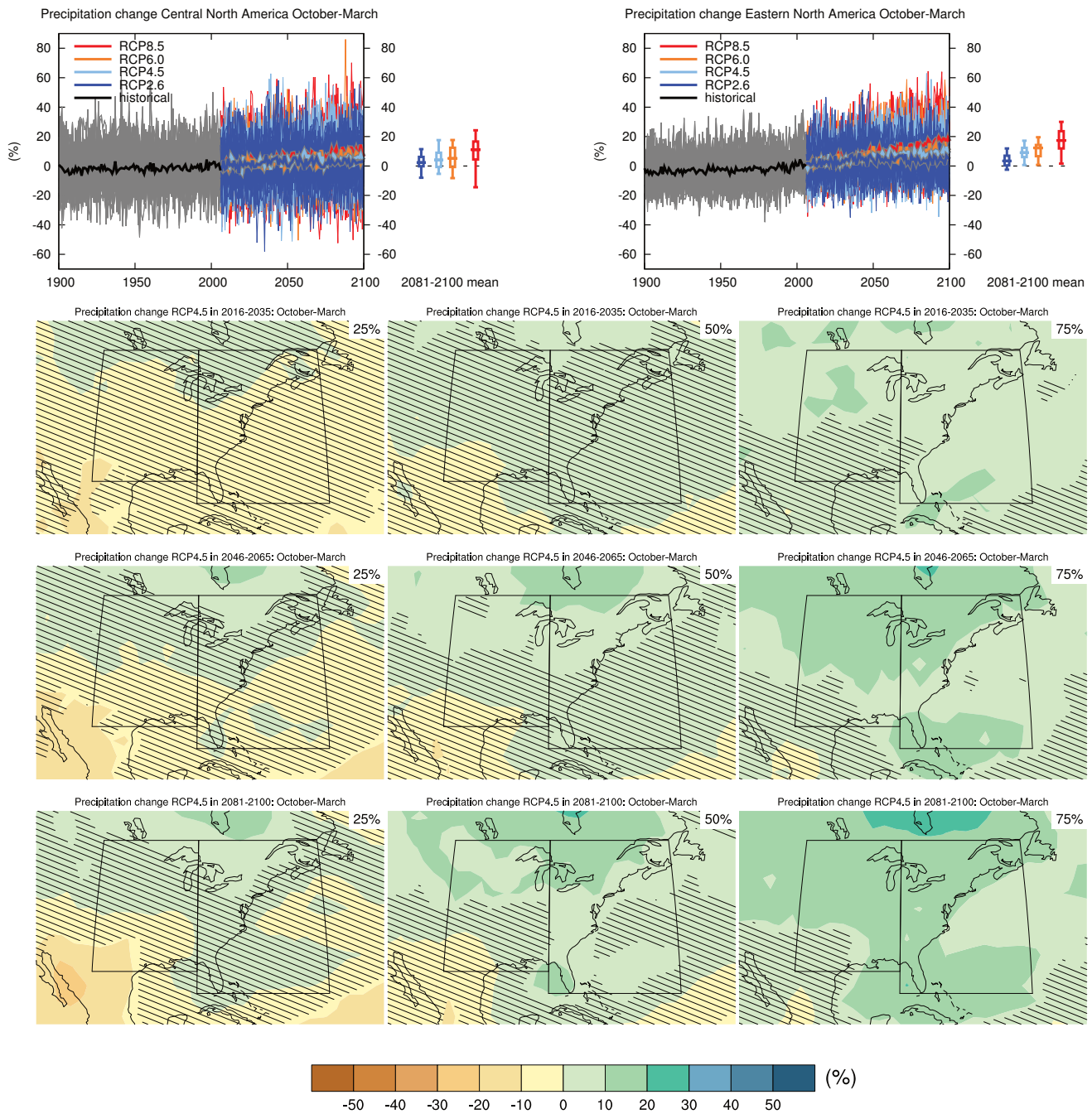
Figure AI.22 | (Top left) Time series of relative change relative to 1986–2005 in precipitation averaged over land grid points in Central North America (28.6°N to 50°N, 105°W to 85°W) in October to March. (Top right) Same for land grid points in Eastern North America (25°N to 50°N, 85°W to 60°W). Thin lines denote one ensemble member per model, thick lines the CMIP5 multi-model mean. On the right-hand side the 5th, 25th, 50th (median), 75th and 95th percentiles of the distribution of 20-year mean changes are given for 2081–2100 in the four RCP scenarios.
