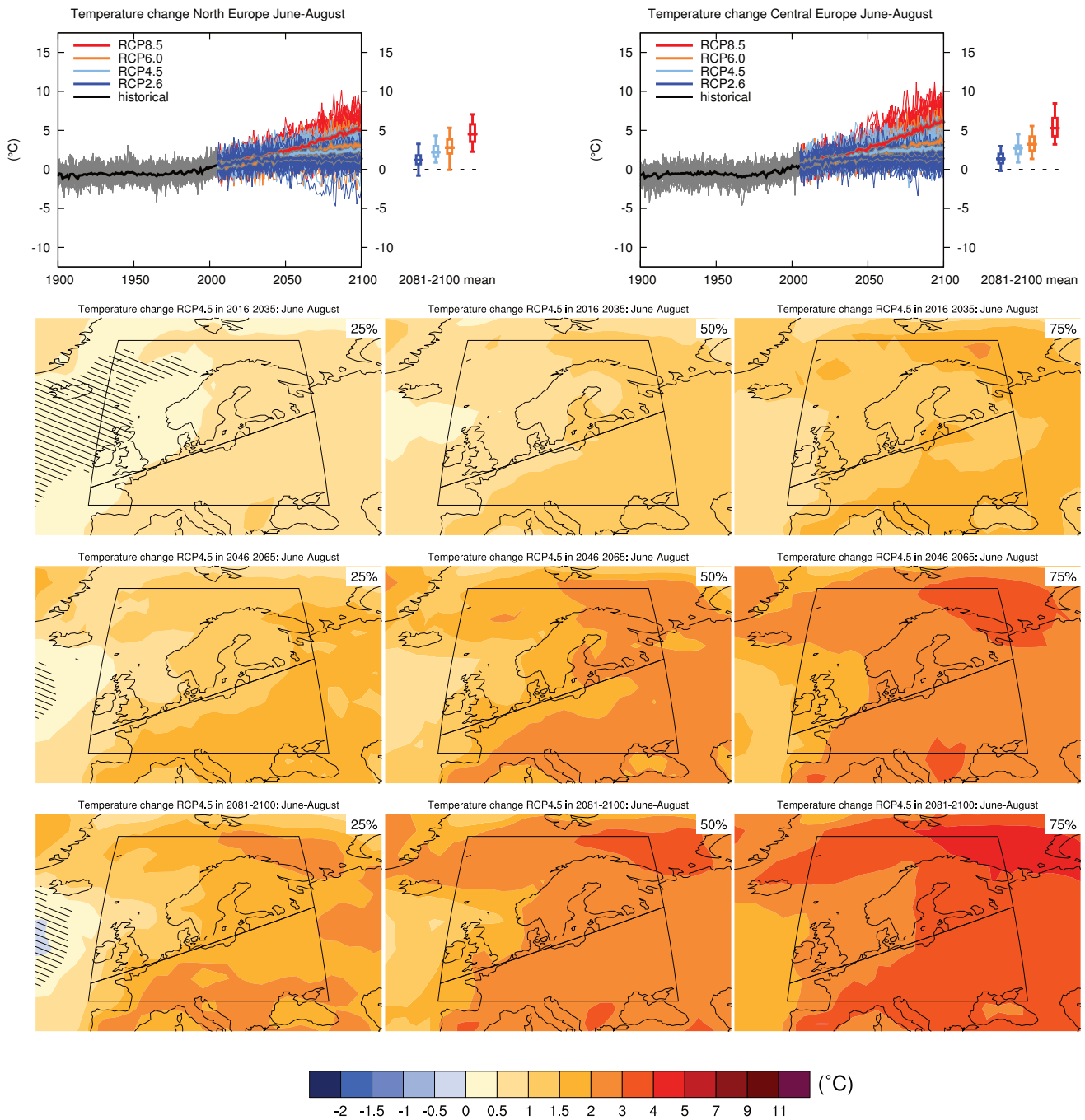
Figure AI.37 | (Top left) Time series of temperature change relative to 1986–2005 averaged over land grid points in North Europe (10°W, 48°N; 10°W, 75°N; 40°E, 75°N; 40°E, 61.3°N) in June to August. (Top right) Same for land grid points in Central Europe (10°W, 45°N; 10°W, 48°N; 40°E, 61.3°N; 40°E, 45°N). Thin lines denote one ensemble member per model, thick lines the CMIP5 multi-model mean. On the right-hand side the 5th, 25th, 50th (median), 75th and 95th percentiles of the distribution of 20-year mean changes are given for 2081–2100 in the four RCP scenarios.
